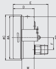
Dimensions (mm)
